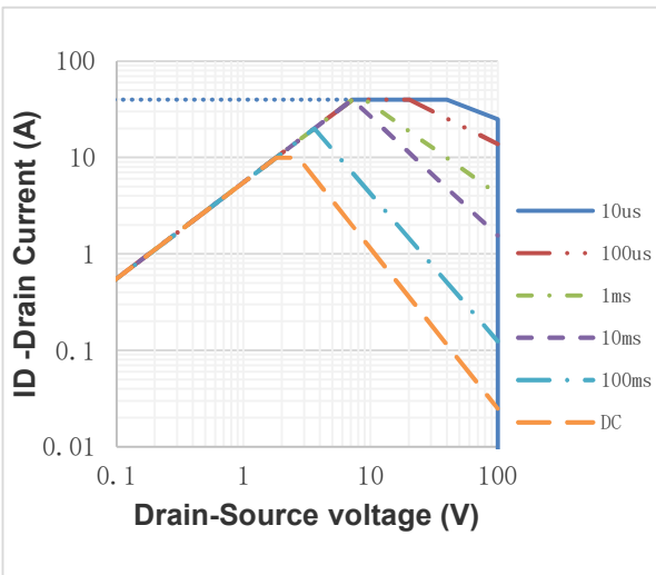
Fig.11 Operating Area
